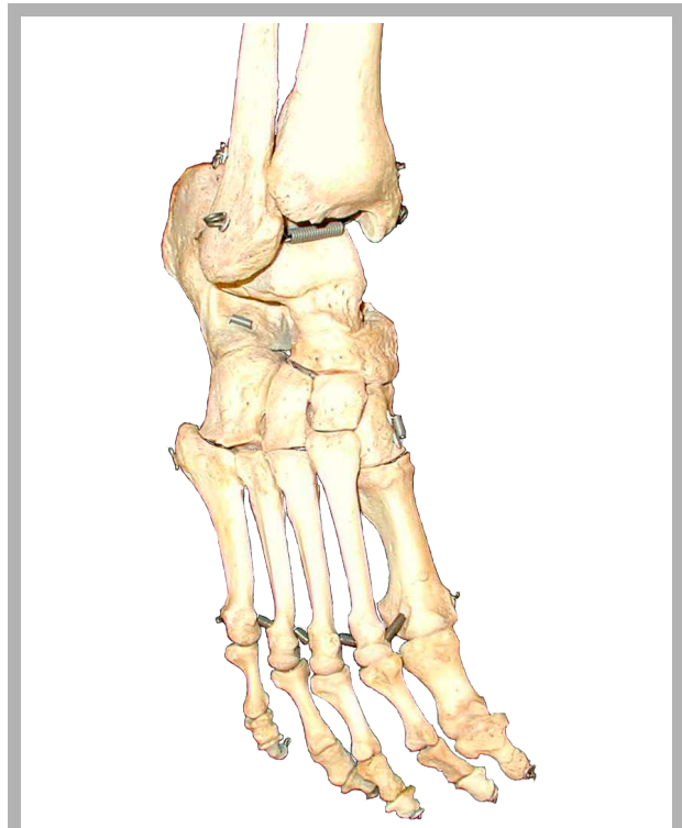
foot skeleton
