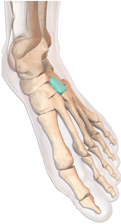
lateral cuneiform
