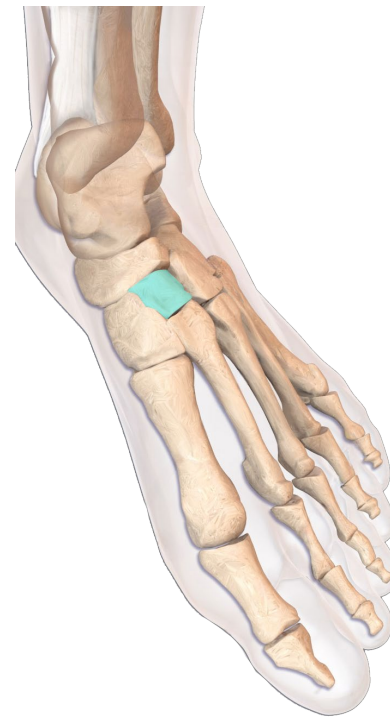
intermediate cuneiform
