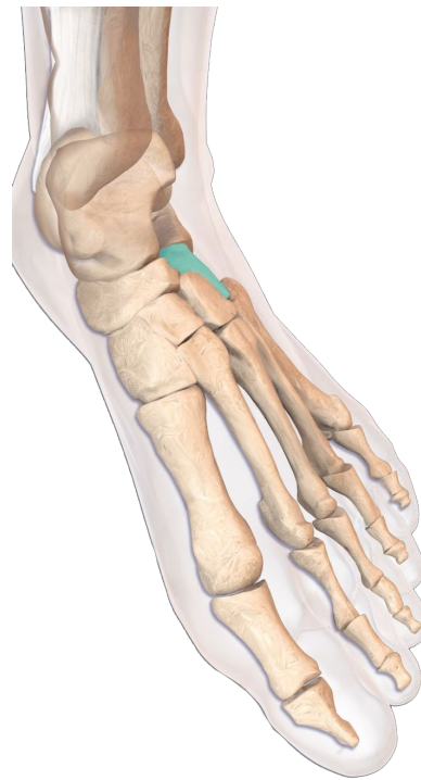
cuboid bone
