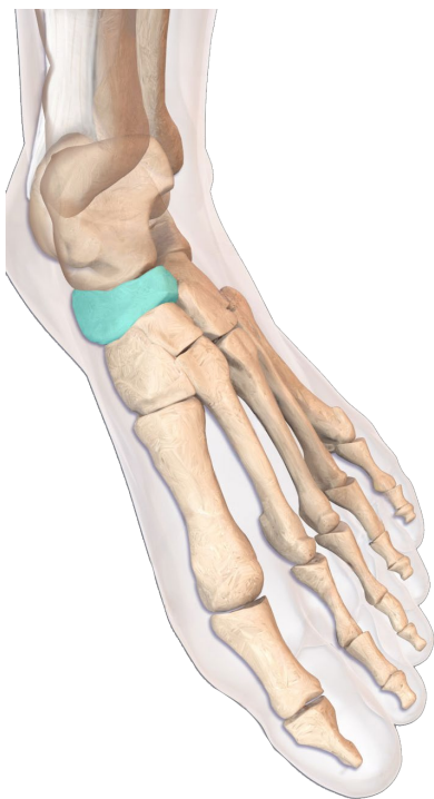
navicular bone
