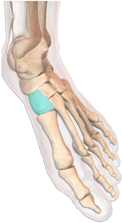
medial cuneiform
