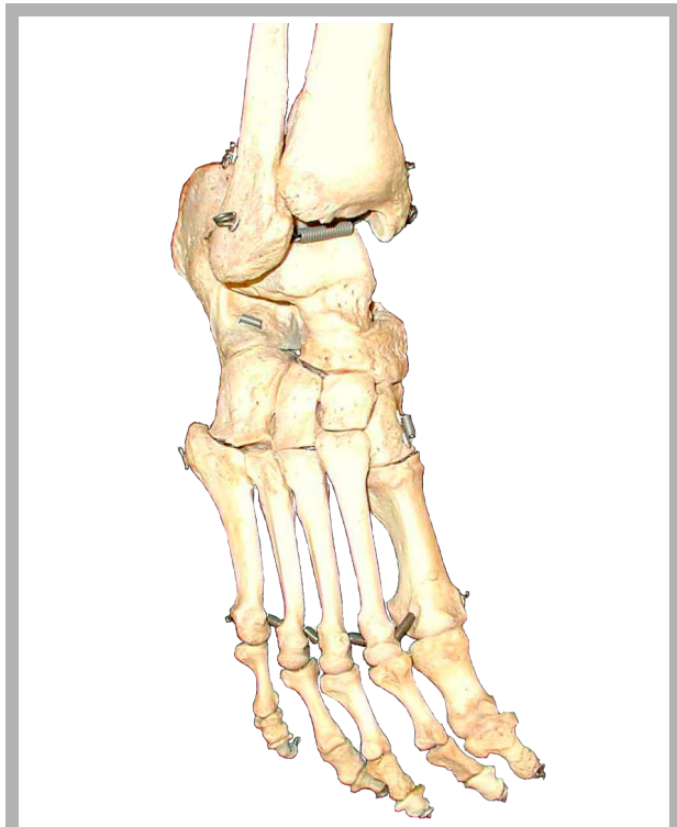
foot skeleton
