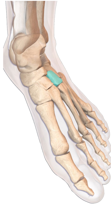
lateral cuneiform
