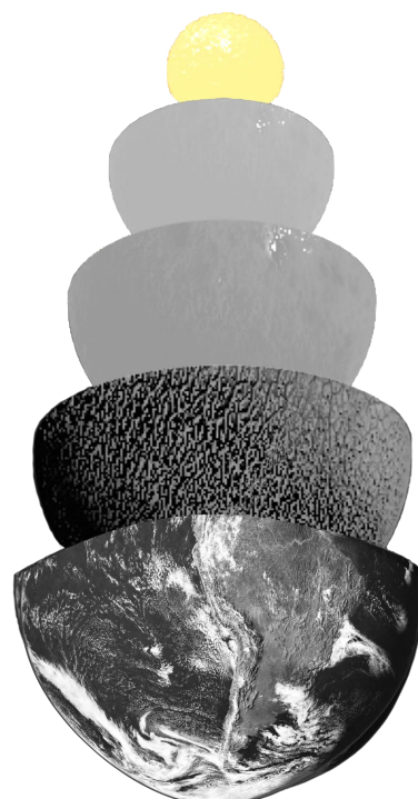
inner core
