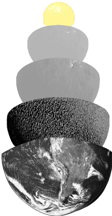
inner core
